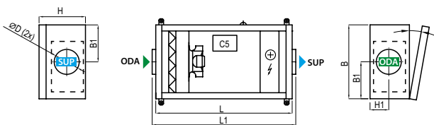
▶ ODA – outdoor intake ▶ SUP – supply air
